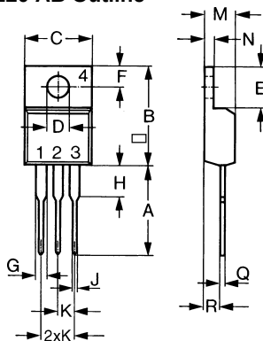
TO-220 AB Outline
