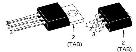
TO-220 AB
