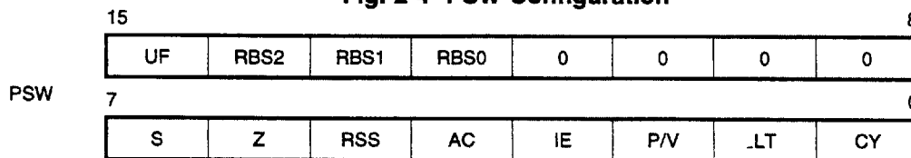
Fig. 2-4 PSW Configuration
