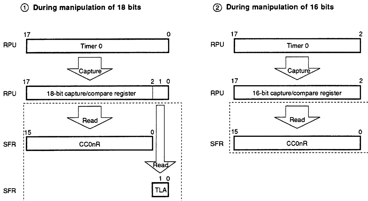
Fig. 4-9 Capture Operation
