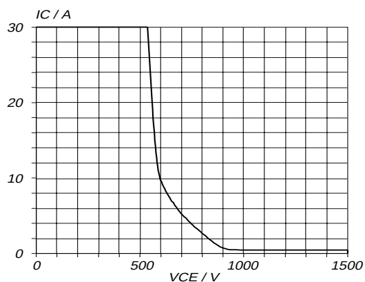
Fig.15. Reverse bias safe operating area. T_j \leq T_{jmax}
