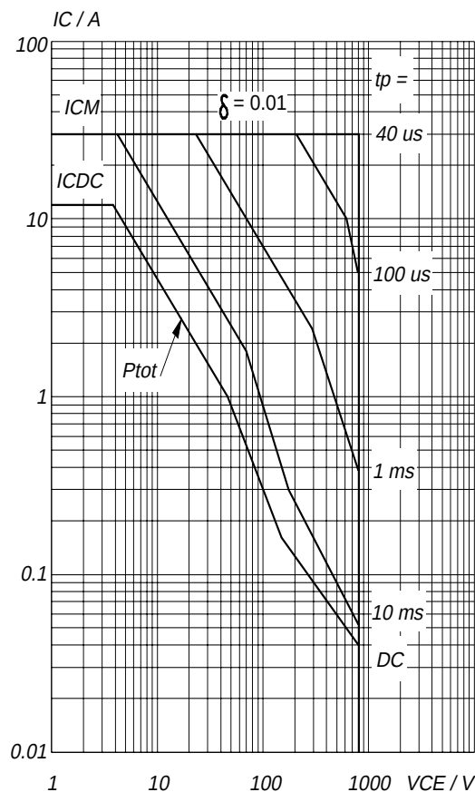
Fig.16. Forward bias safe operating area. T_{hs} = 25^\circ\text{C} I_{CDC} & I_{CM} = f(V_{CE}) ; I_{CM} single pulse; parameter t_p Second-breakdown limits independent of temperature. Mounted with heatsink compound.
