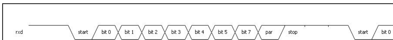
Figure 5.1 UART Receive Waveform
