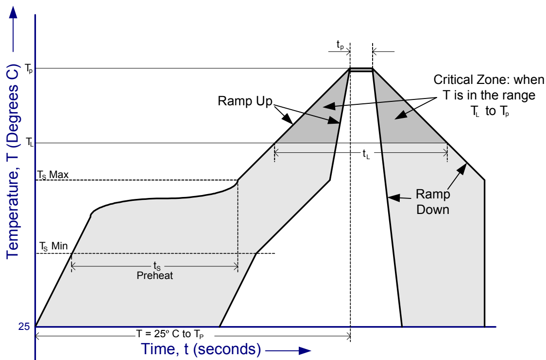
Figure 8.2 VNC1L Solder Reflow Profile
