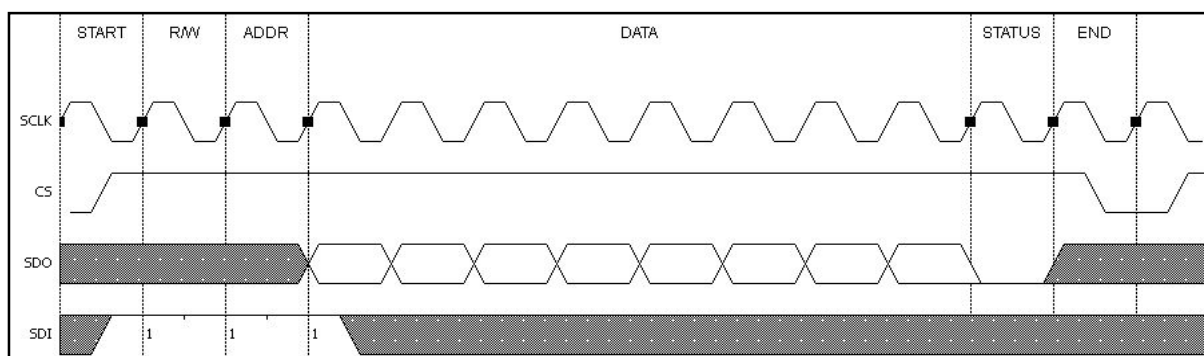
Figure 5.6 SPI Slave Mode Status Read
