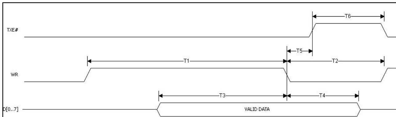
Figure 5.8 FIFO Write Cycle
