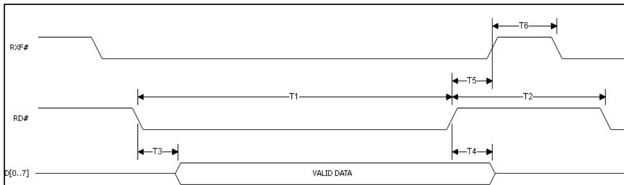
Figure 5.7 FIFO Read Cycle
